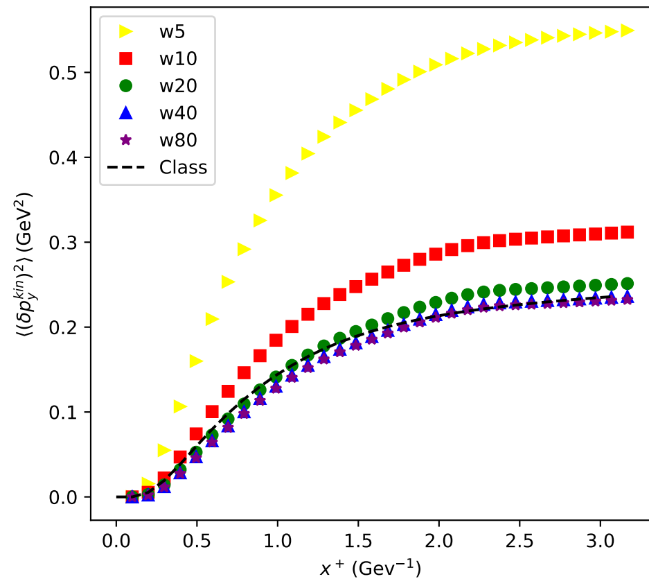
L=5 fm, Kinetic momentum broadening
