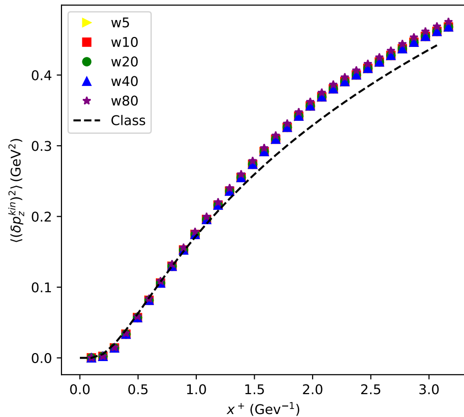
L=5 fm, Kinetic momentum broadening
